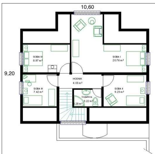
MANSARDA
