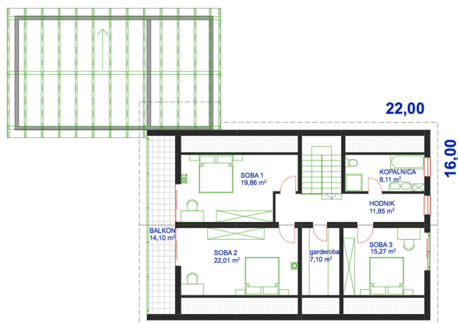
MANSARDA
