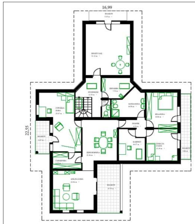
MANSARDA
