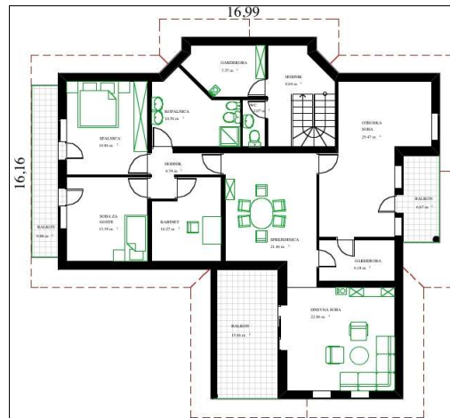
MANSARDA
