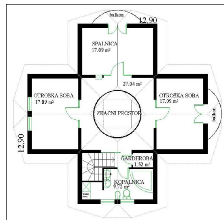
MANSARDA
